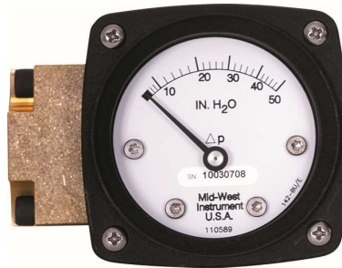
2-1/2" Dial 0-50" H2O
