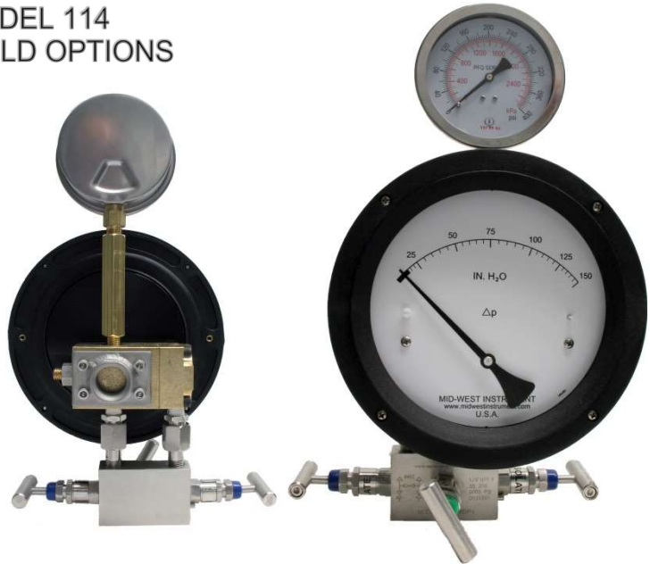
Model 114 w/6" Dial mounted to Model 113343 3-Valve Mini-Manifold 1/4" FNPT Process connections Show with optional stand-off & pressure gauge
